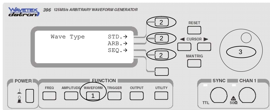
Figure 3-5. Selecting Waveform Type
