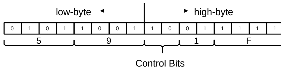
Figure 4-7. Terminating the DMA mode with the MSB Control bit set to “1”
