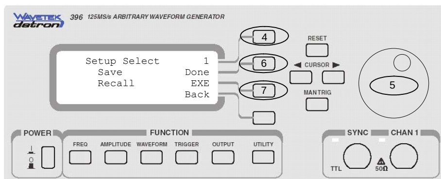
Figure 3-29. Saving and Recalling Setups
