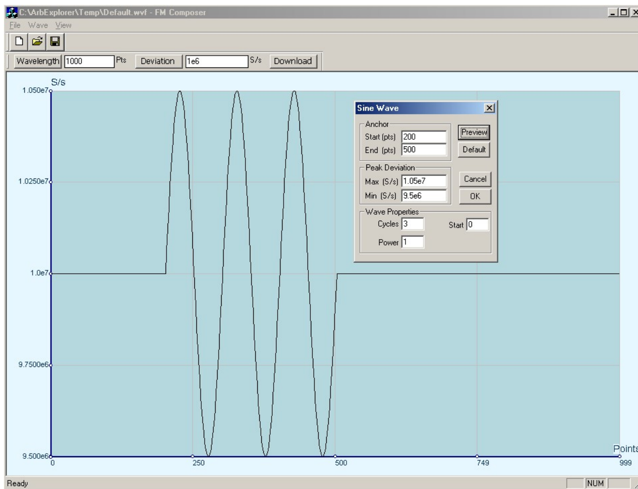
Figure 5-19. An Example of Generating Modulating Sine Using the Built-in Library.
